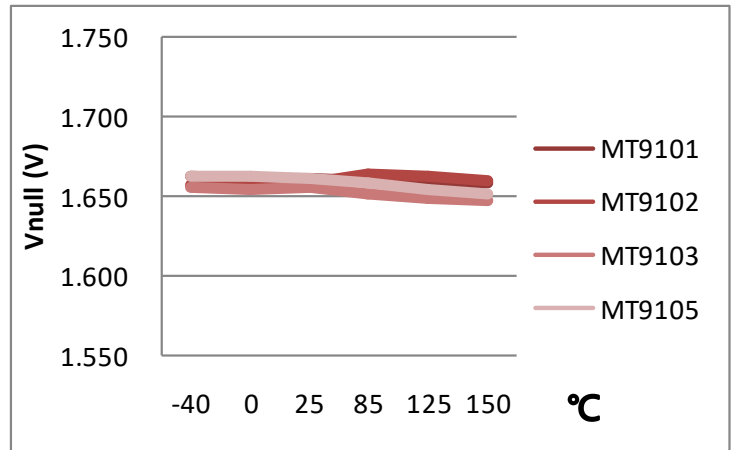
Figure.9 Vnull vs. Temperature (At Vcc=3.3V)
