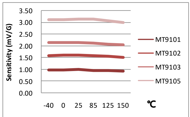
Figure.11 Sensitivity vs. Temperature (At Vcc=3.3V)
